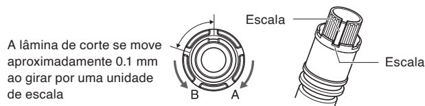
PHP35-CB09-HS/PHP35-CB15-HS
